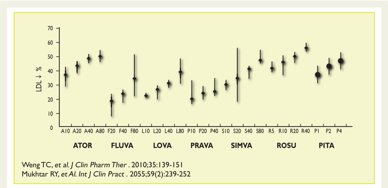
Supplementary Figure A A systematic review and meta-analysis of the therapeutic equivalence of statins. ATOR = atorvastatin; FLUVA = fluvastatin; LOVA = lovastatin; PRAVA = pravastatin; SIMVA = simvastatin; ROSU = rosuvastatin; PITA = pitavastatin.
